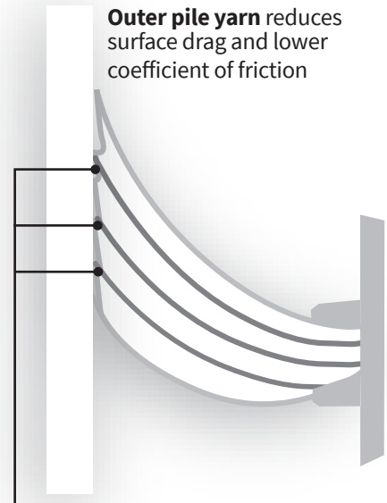
Three fins encapsulated by yarn provides superior sealing and compression set resistance
